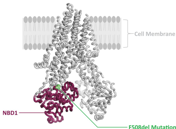
Figure 1. CFTR Structure
