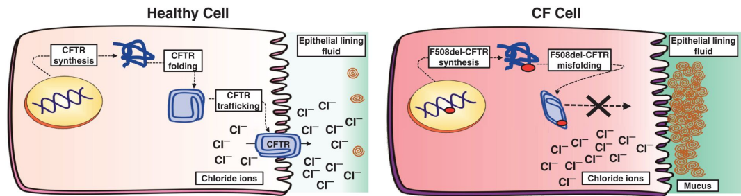
Figure 5. CFTR Regulates Chloride Transport in Epithelial Cells
