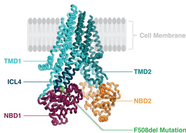
Figure 6. The CFTR Protein and the F508del Mutation
