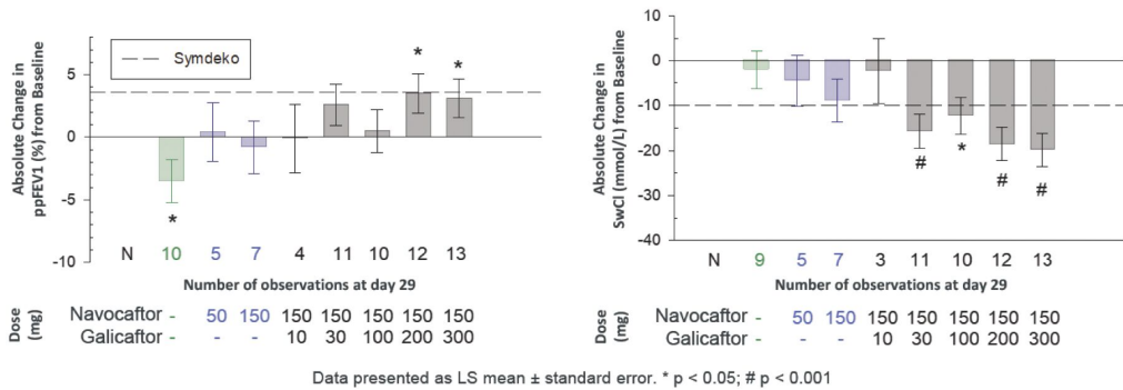
Figure 25. Galicaftor + Navocaftor Combination Showed Similar Activity to Symdeko in Phase 2 Cross-Trial Comparison
