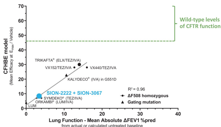
Figure 13. CFHBE Model Correlates to Improved Lung Function
