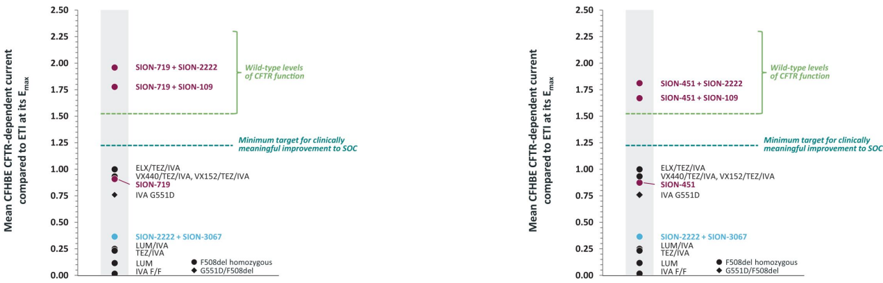
Figure 22. SION-719 and SION-451 Combinations with Galicaftor or SION-109 Were Highly Active in the CFHBE Model at E_{max}
